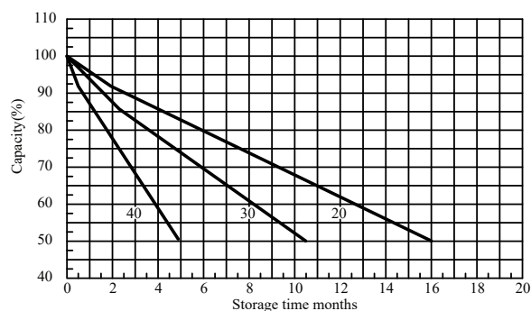
Self-discharge characteristic
